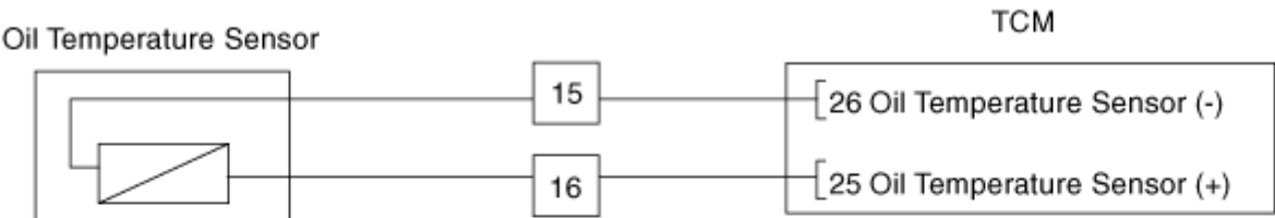
[Circuit Diagram]
