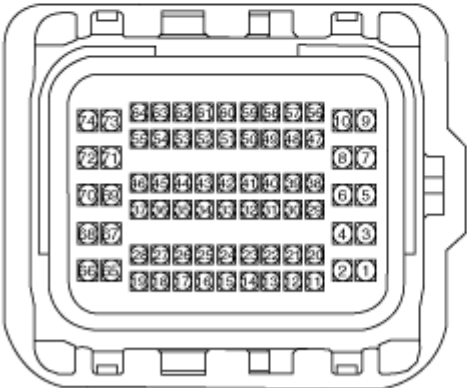
[TCM Connector]
