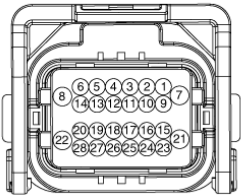
[Main Connector]
